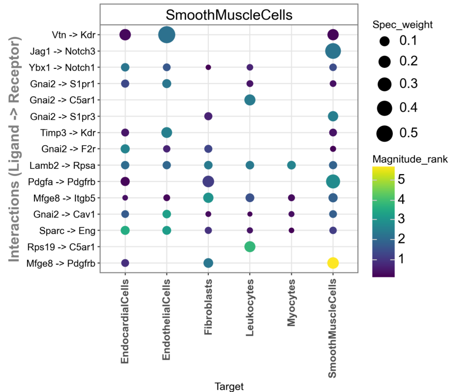
SmoothMuscleCells as senders -- 30m
