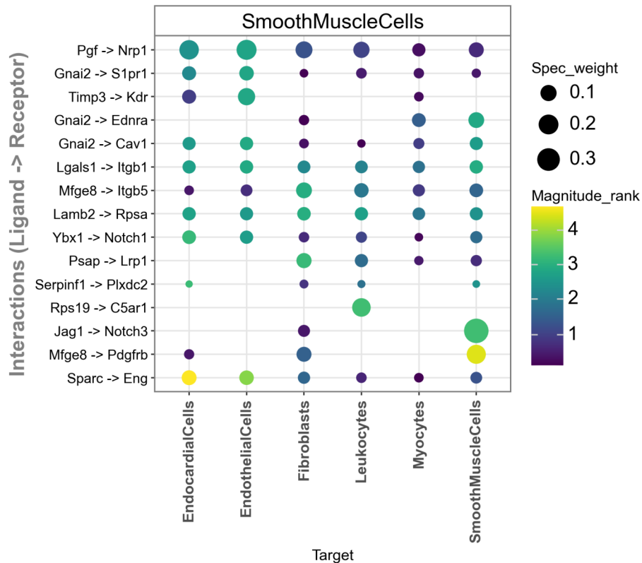
SmoothMuscleCells as senders -- 3m
