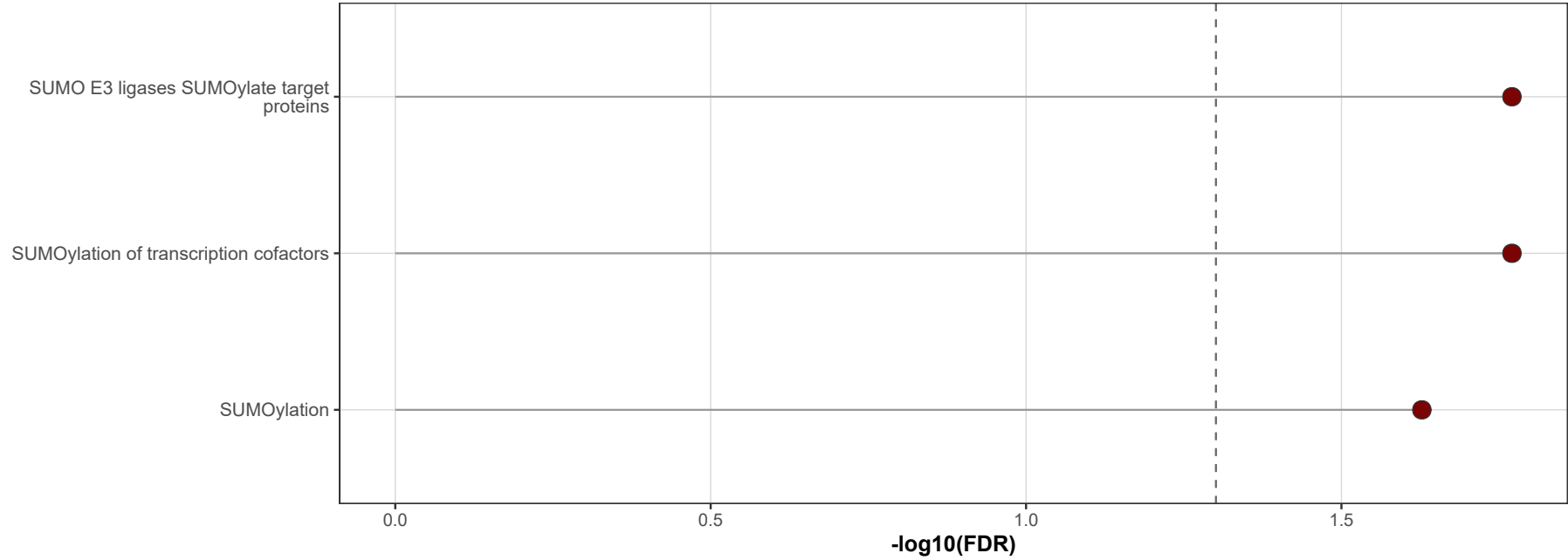
Reactome - Top Significance
