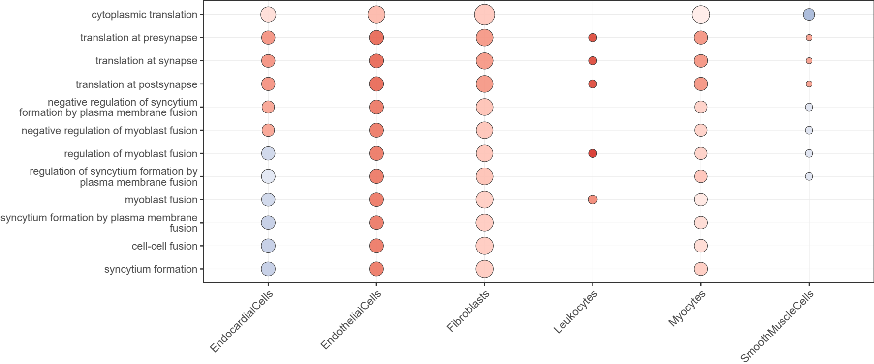
GO_BP - Top Significance
