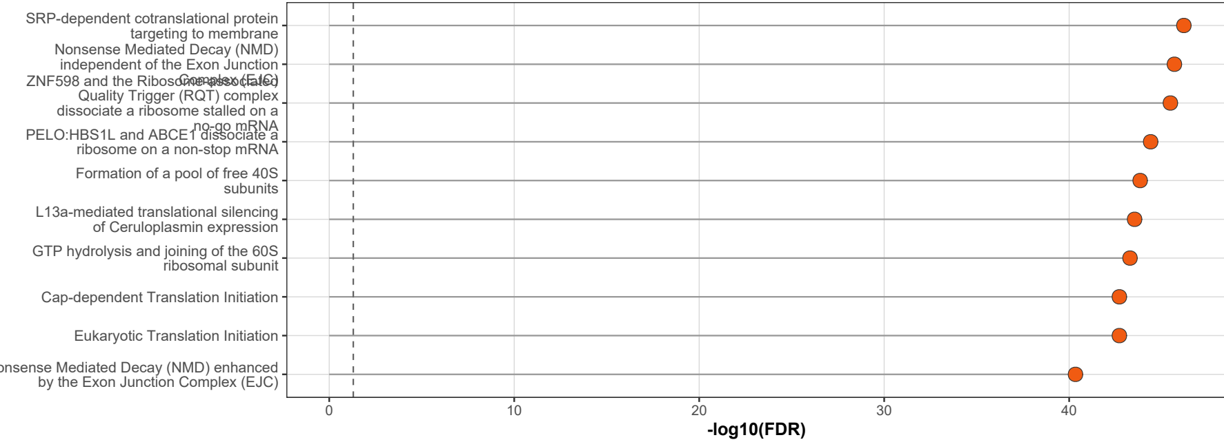
Reactome - Top Significance
