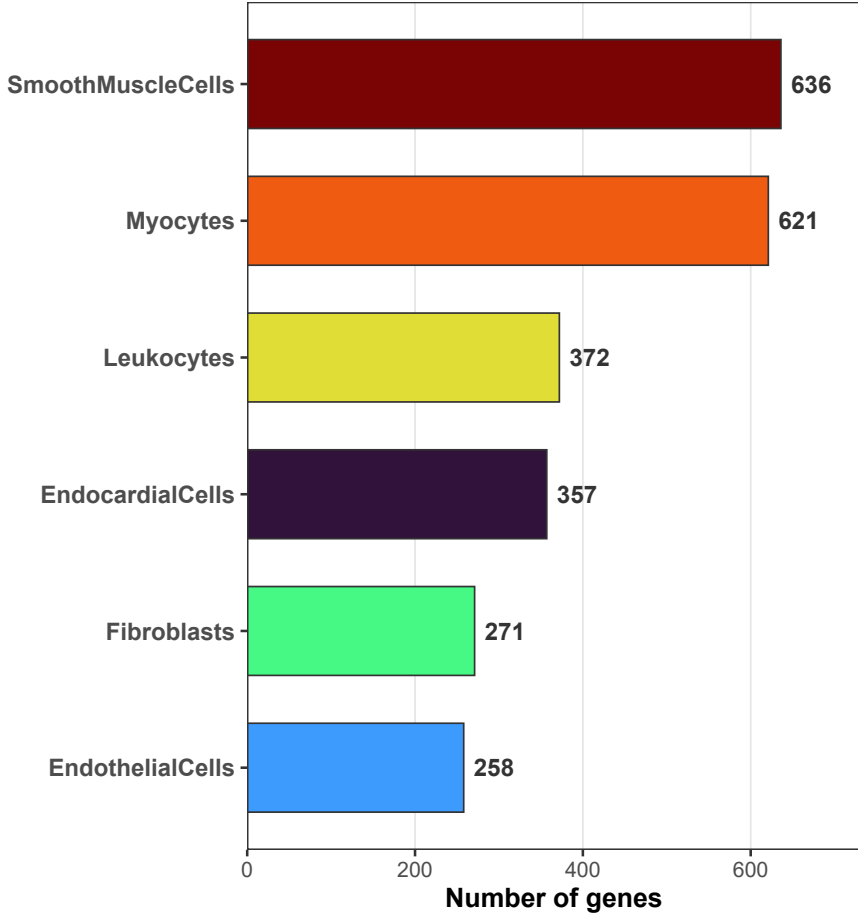
Reactome - Enriched Terms
