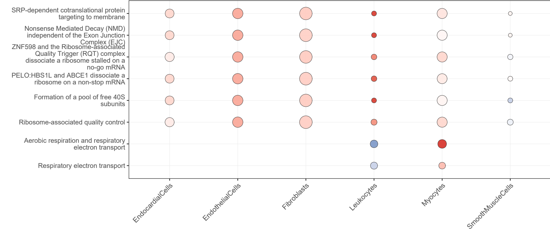
Reactome - Top Significance
