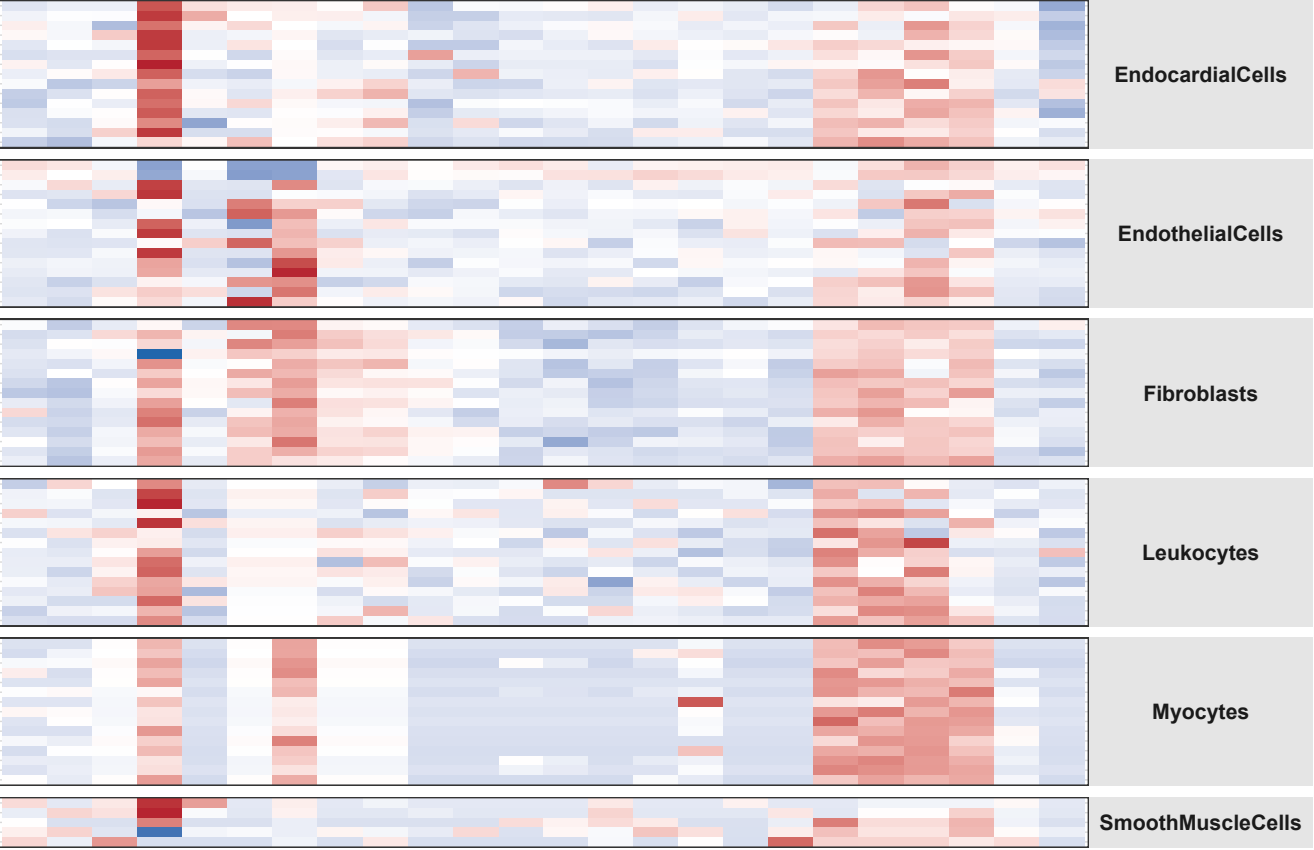
Expression heatmap by cell type
