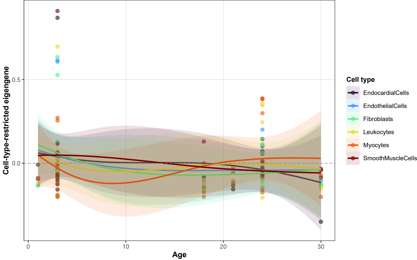
Module darkgreen -- trajectory by cell type
