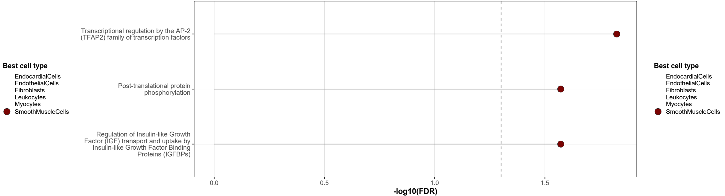
Reactome - Top Significance
