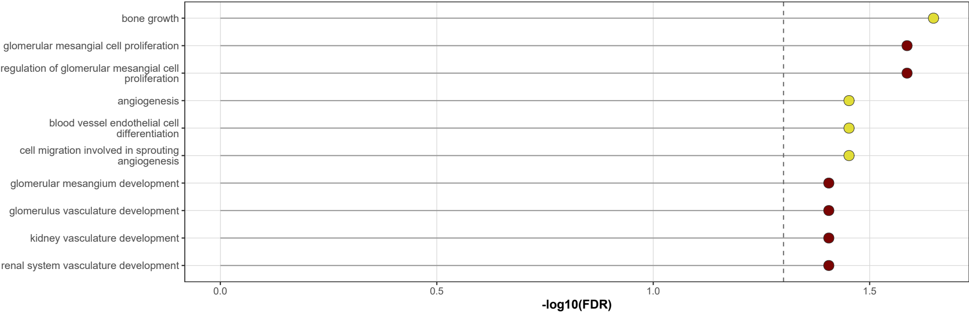
GO_BP - Top Significance
