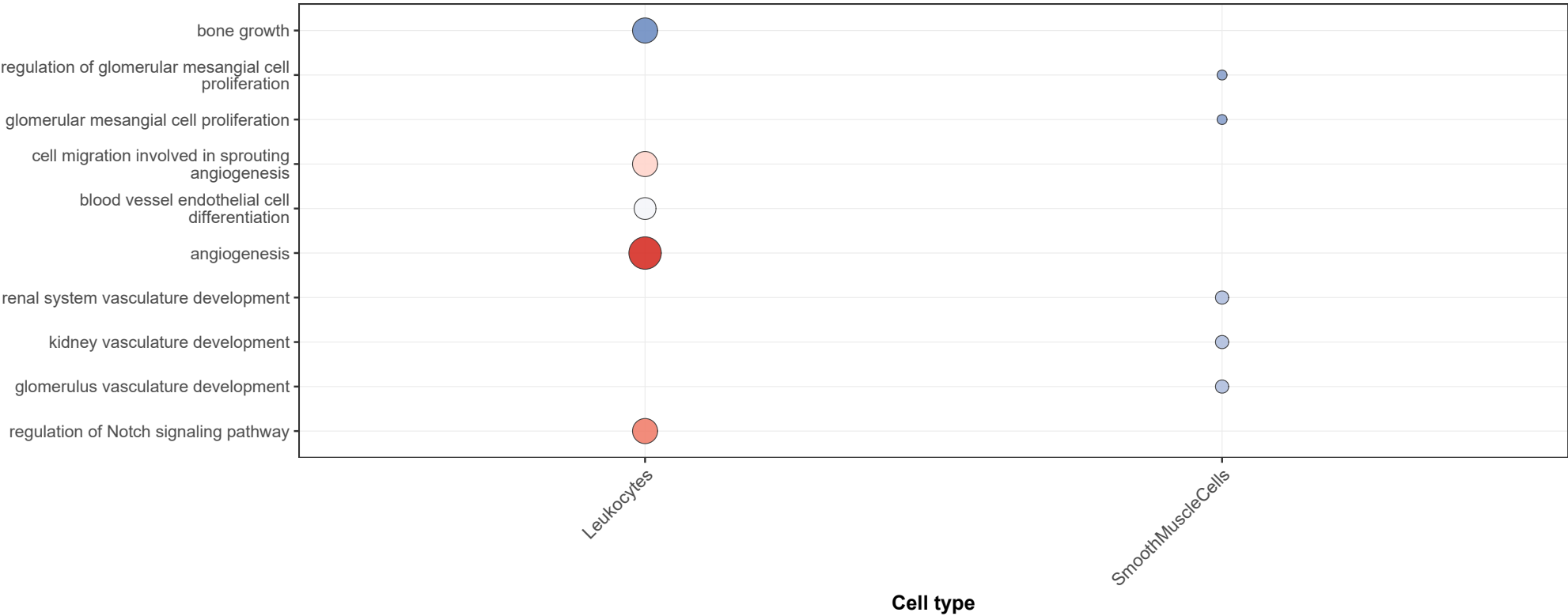
GO_BP - Top Significance
