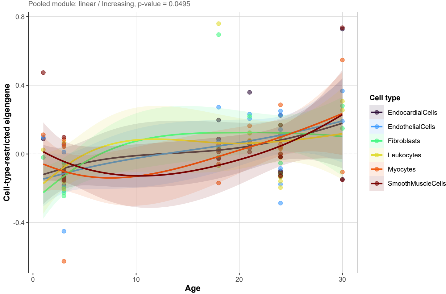
Module darkorange -- trajectory by cell type
