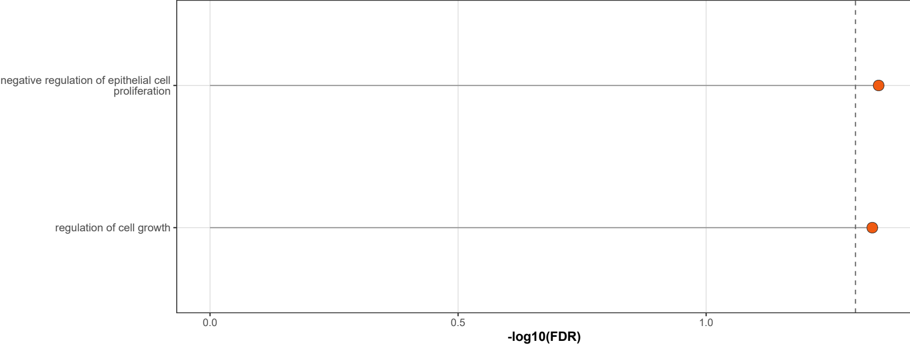
GO_BP - Top Significance
