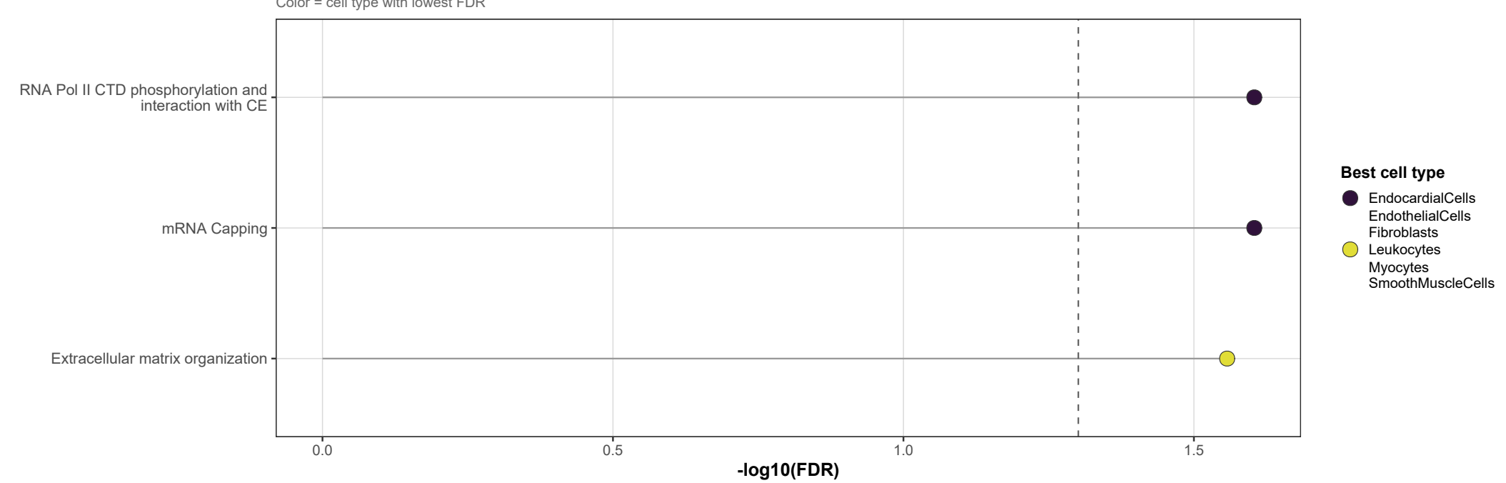
Reactome - Top Significance
