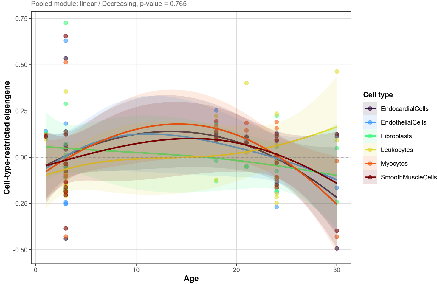
Module darkred -- trajectory by cell type
