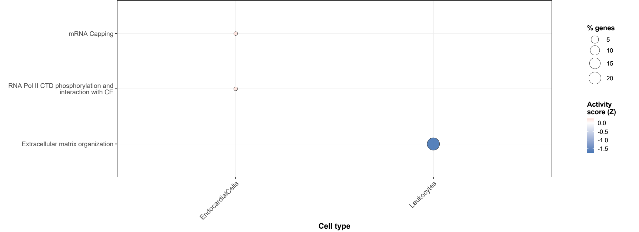
Reactome - Top Significance
