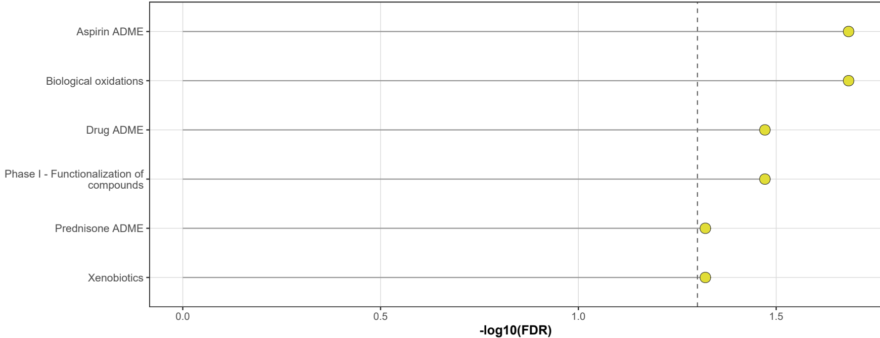
Reactome - Top Significance
