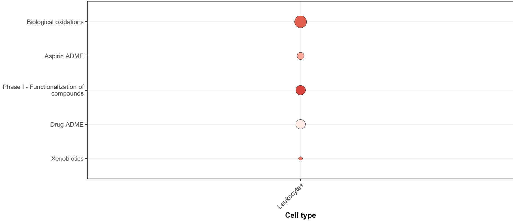
Reactome - Top Significance
