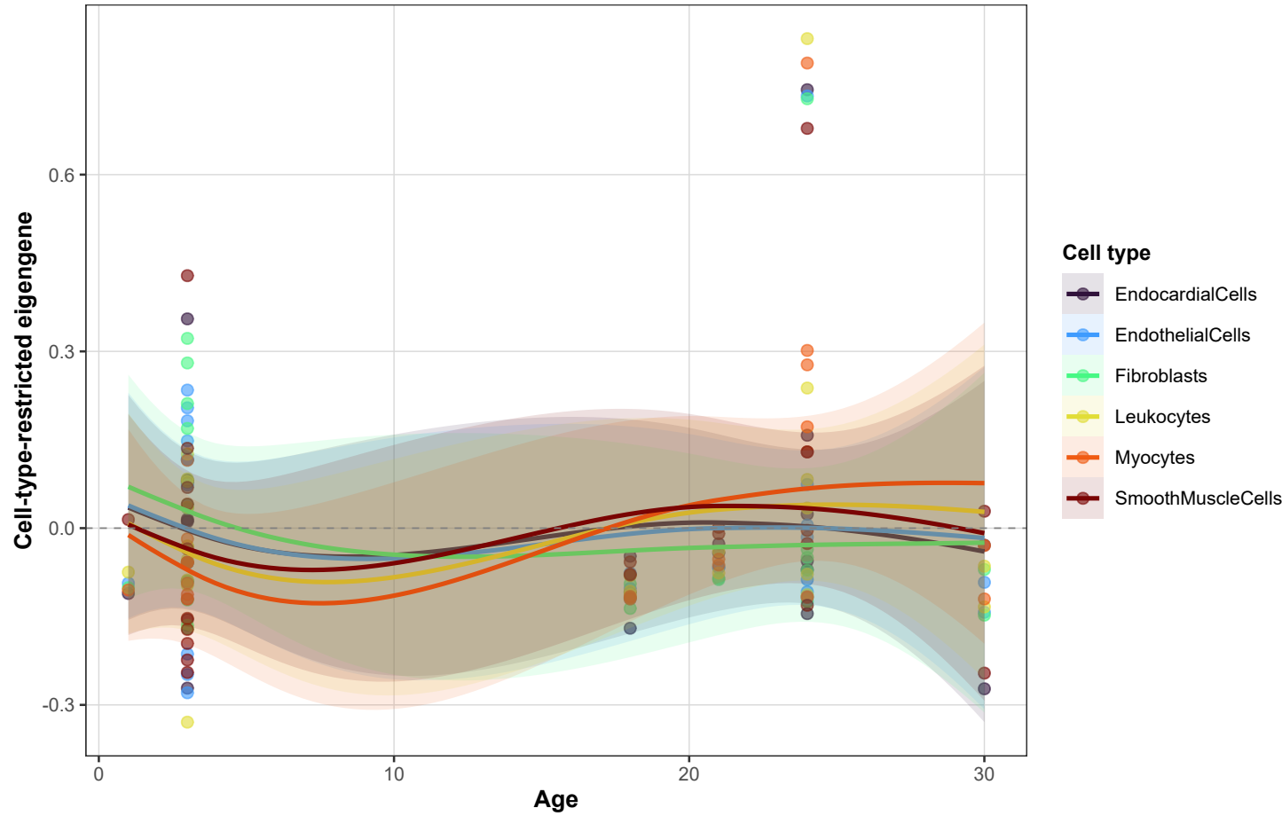
Module darkturquoise -- trajectory by cell type
