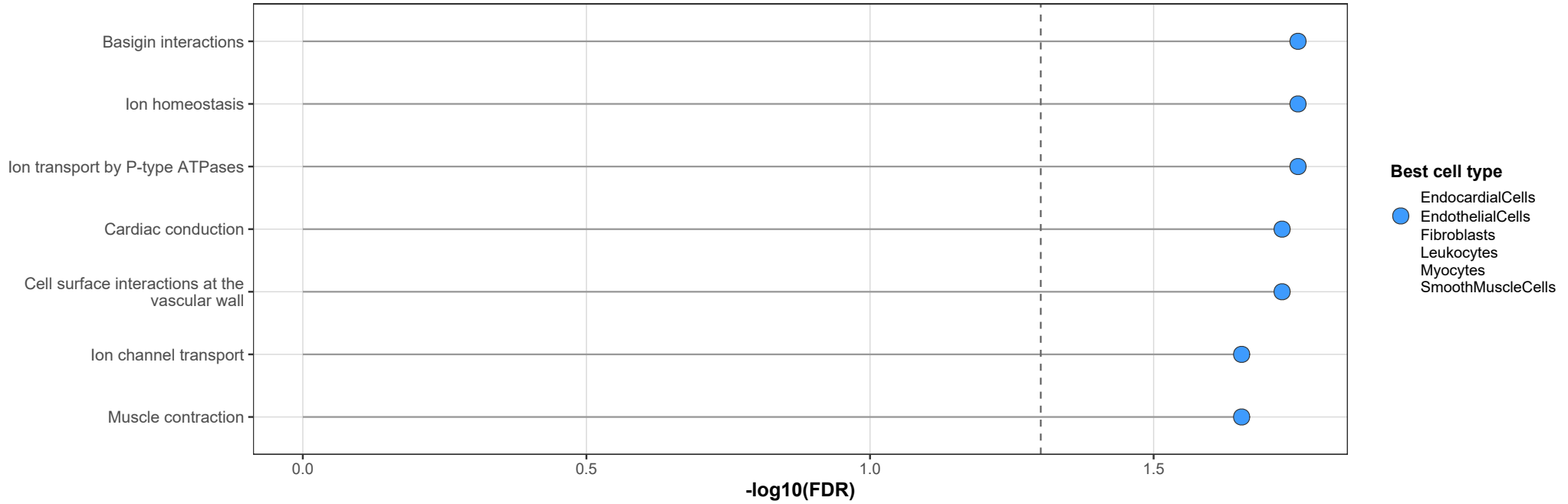
Reactome - Top Significance
