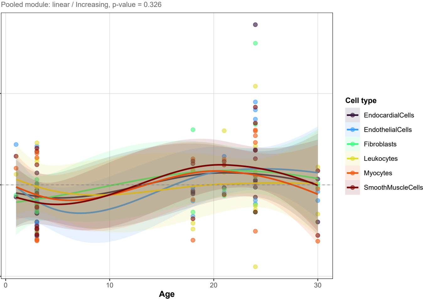
Module magenta -- trajectory by cell type
