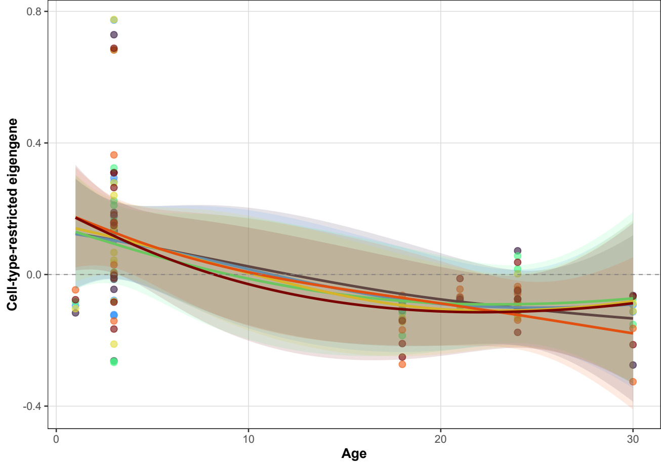
Module midnightblue -- trajectory by cell type
