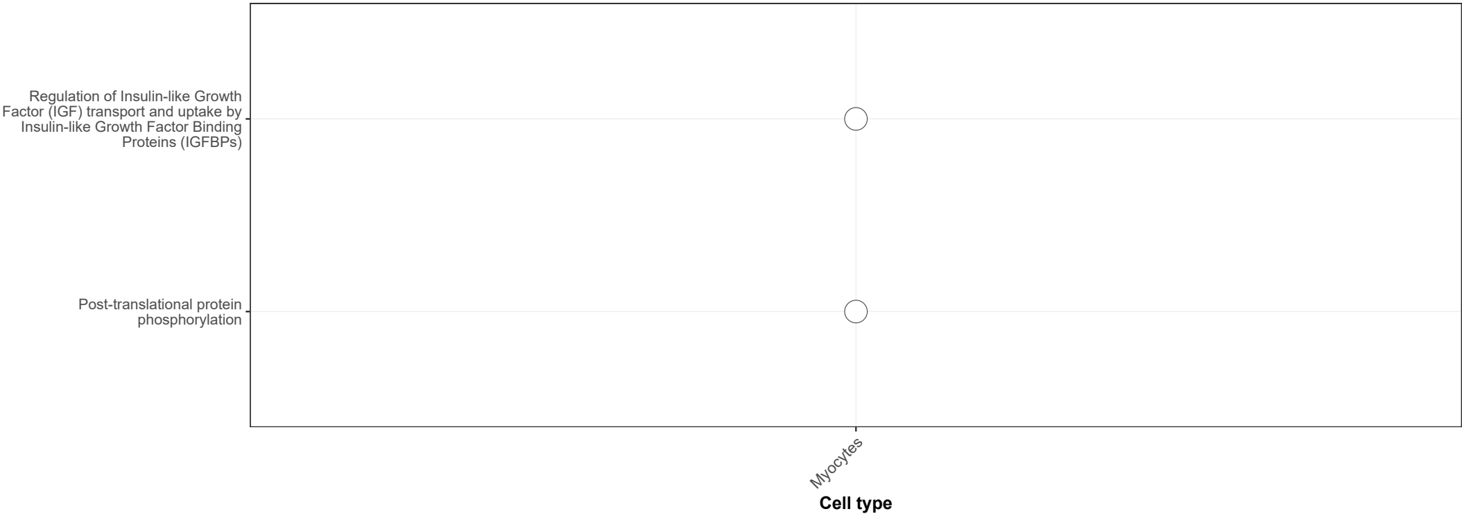
Reactome - Top Significance
