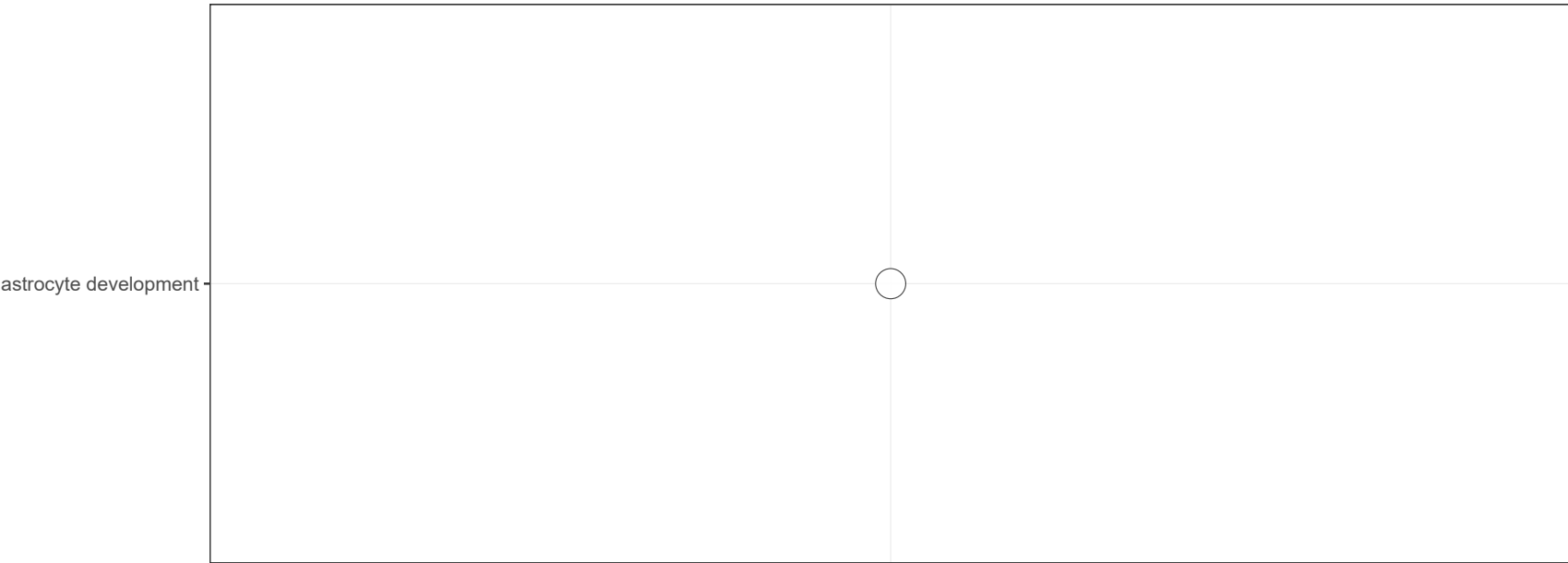
GO_BP - Enriched Terms
