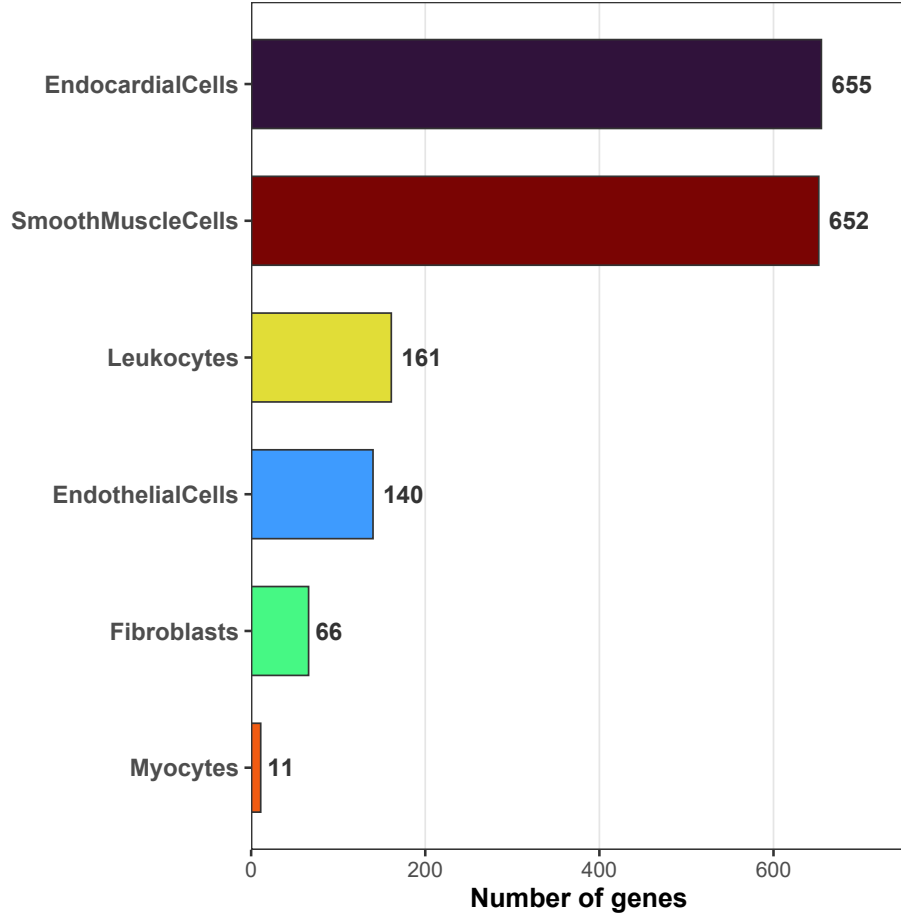
Reactome - Enriched Terms
