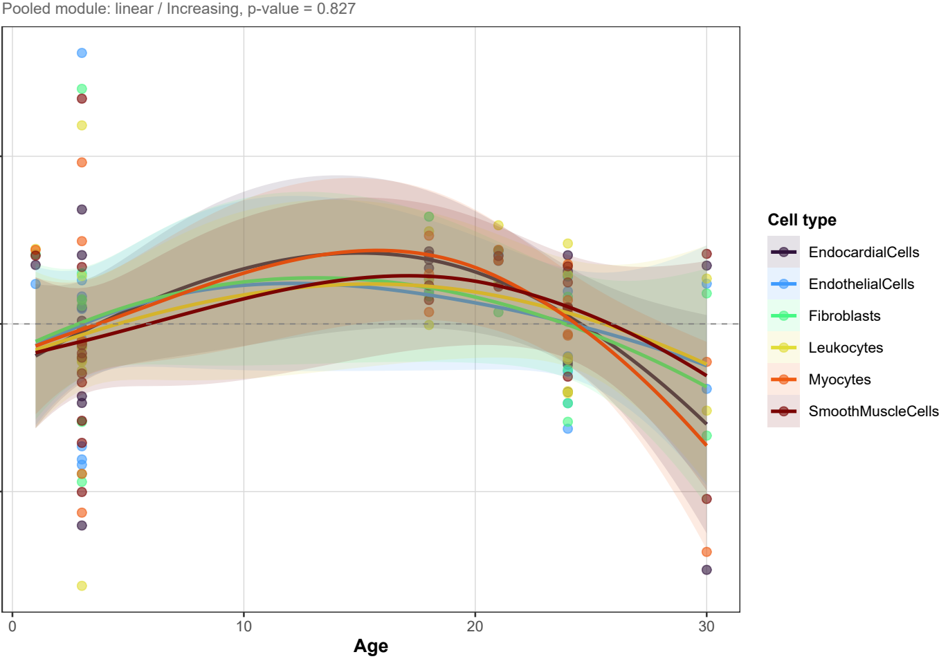
Module red -- trajectory by cell type
