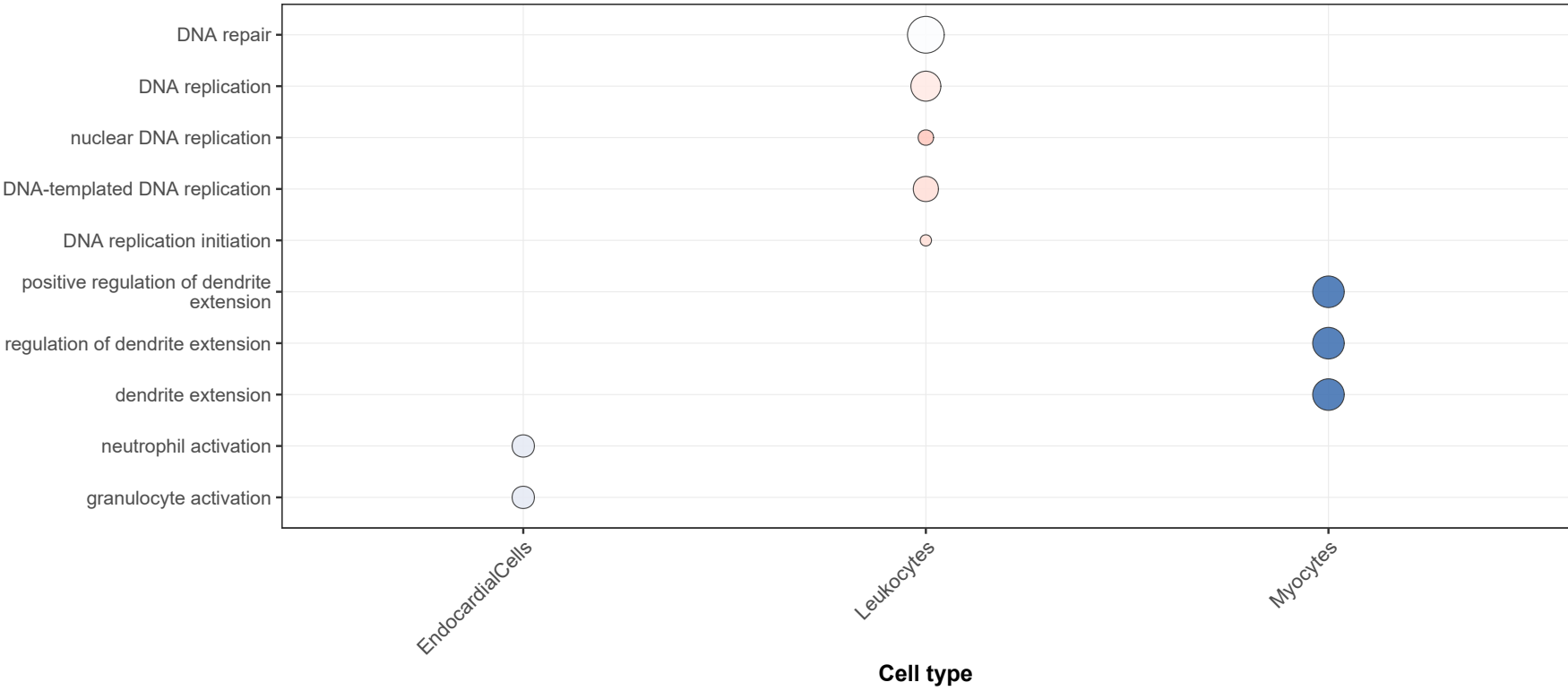
GO_BP - Top Significance
