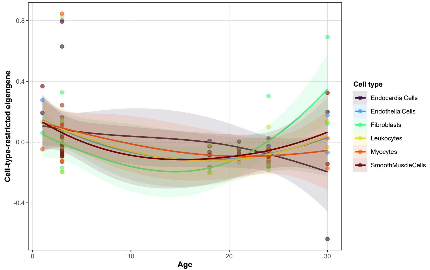
Module sienna3 -- trajectory by cell type
