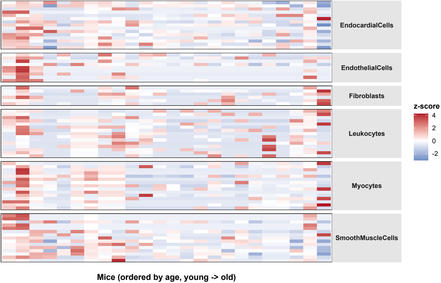
GO_BP - Enriched Terms
