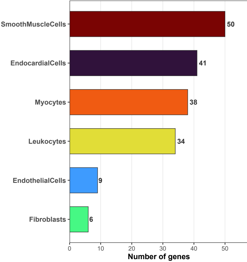
Reactome - Enriched Terms
