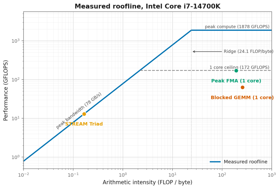
Figure 5.4: Measured roofline with all core and single core compute ceilings.
