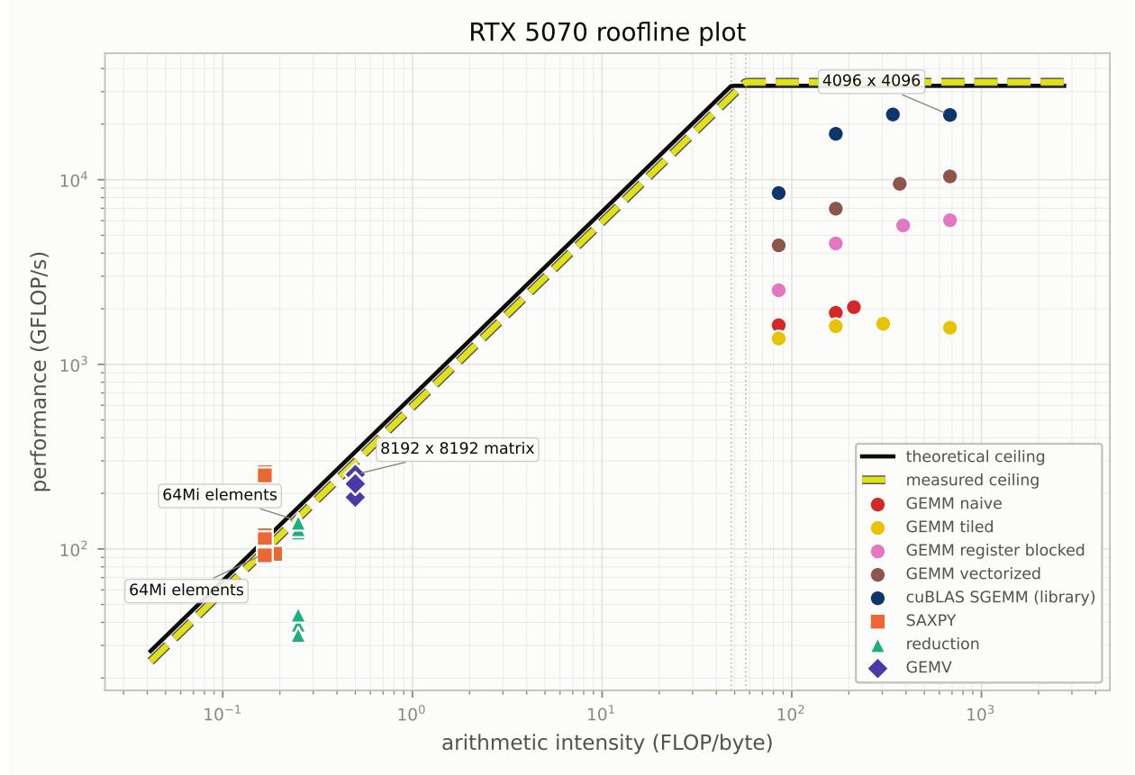
Figure 1: Kernel ladder on the RTX 5070 roofline, theoretical and measured ceilings shown together. One label per kernel family gives the largest problem size that family was run at.
