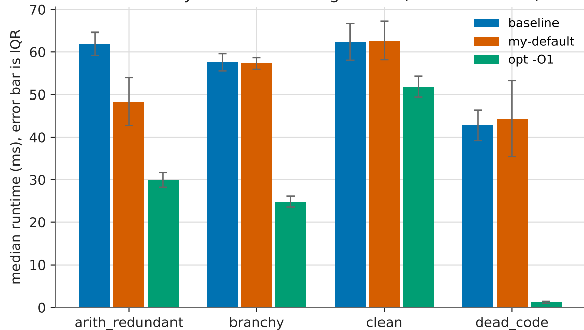
Runtime by kernel and configuration (backend at -O0)
