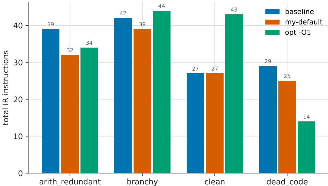
IR instruction count by kernel and configuration
