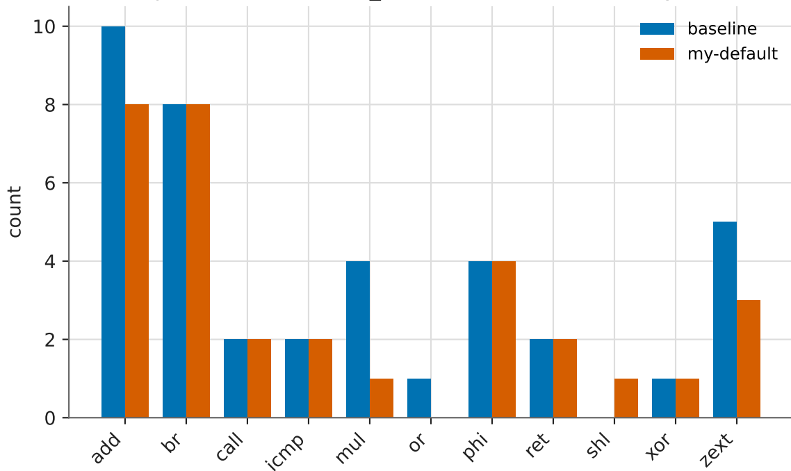
Per opcode counts, arith_redundant: baseline vs my-default
