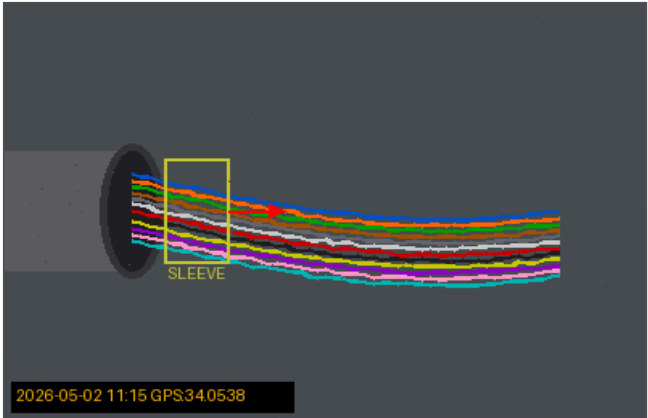
PHOTO 2: Cable Stress Point Micro-bend at conduit entry. Sleeve displaced 8cm. Micro-bend source.
