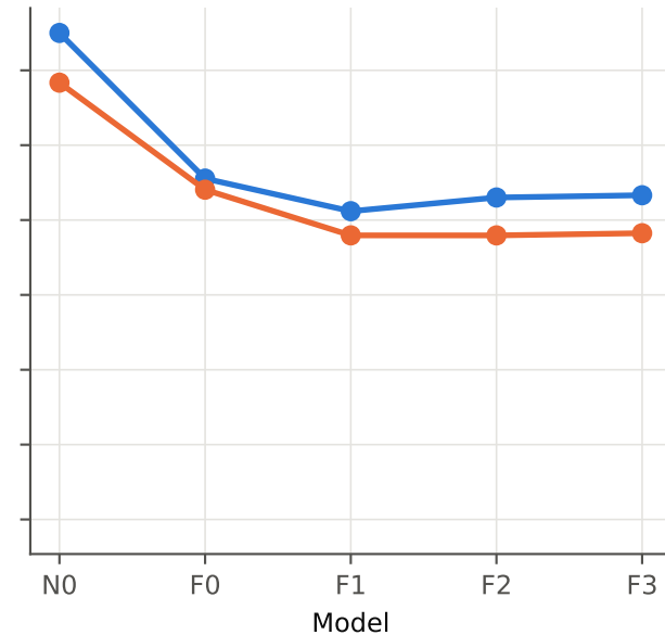
Robustness: 2024 only
