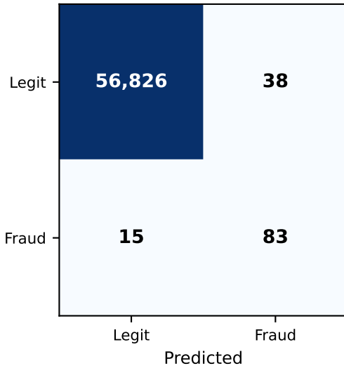
LR
