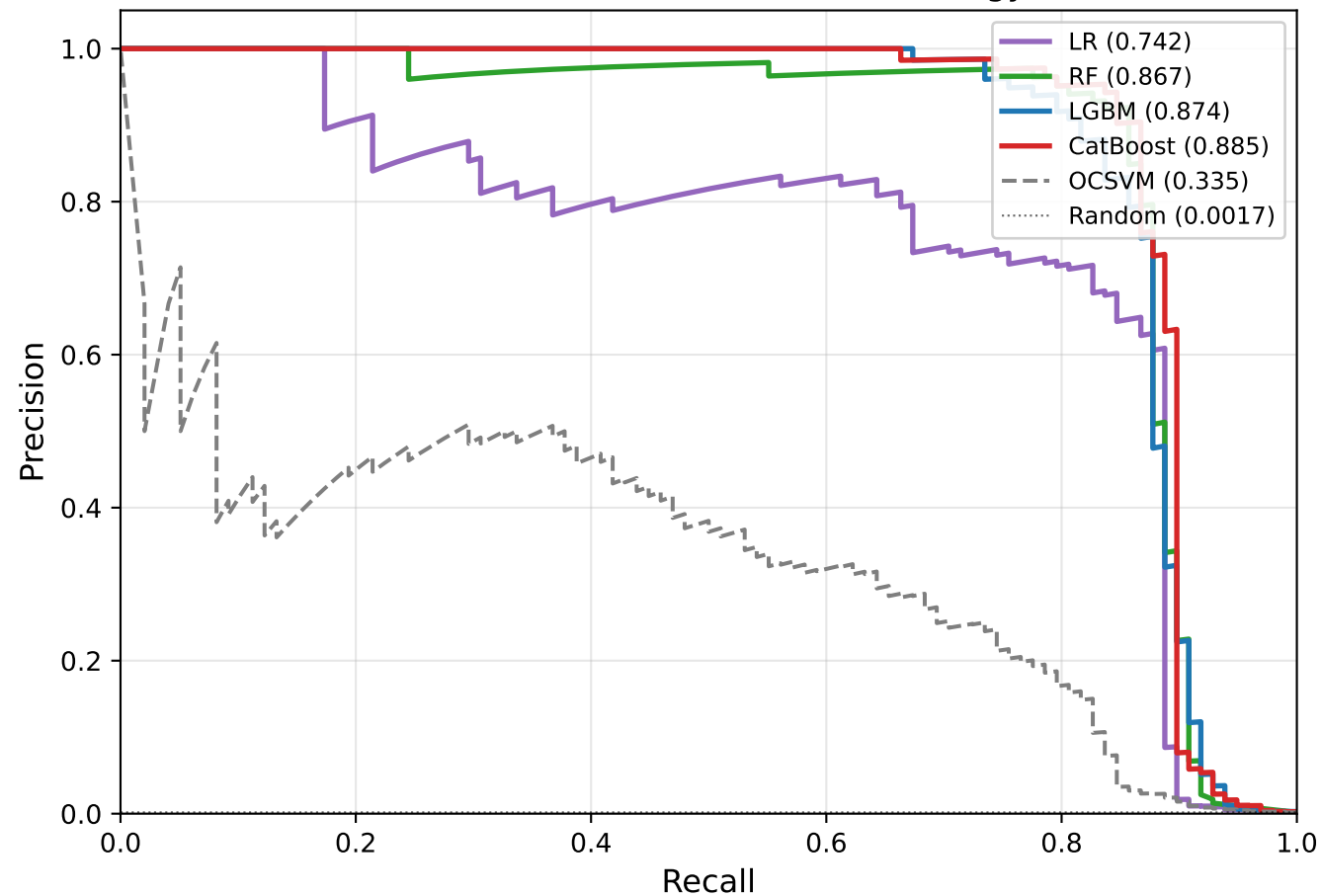
Precision-Recall Curves — ULB 2013 (strategy = None)
