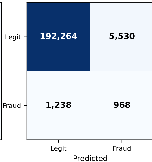
LGBM
