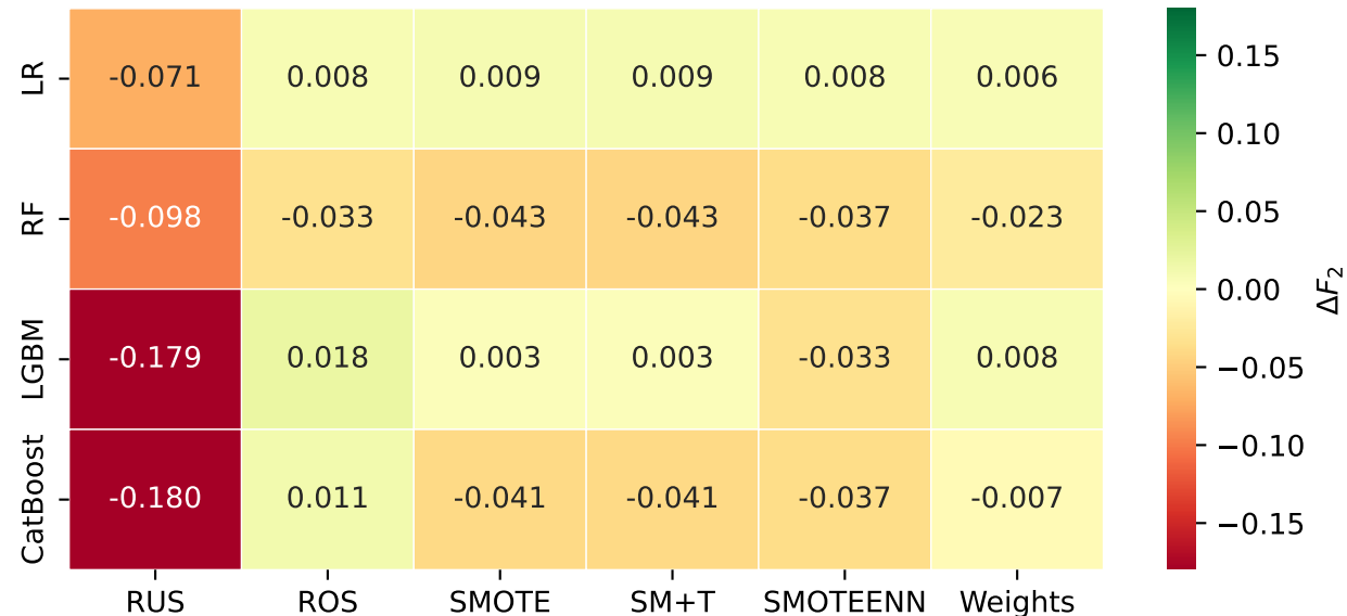
\Delta F_2 (strategy – None) — ULB 2013
