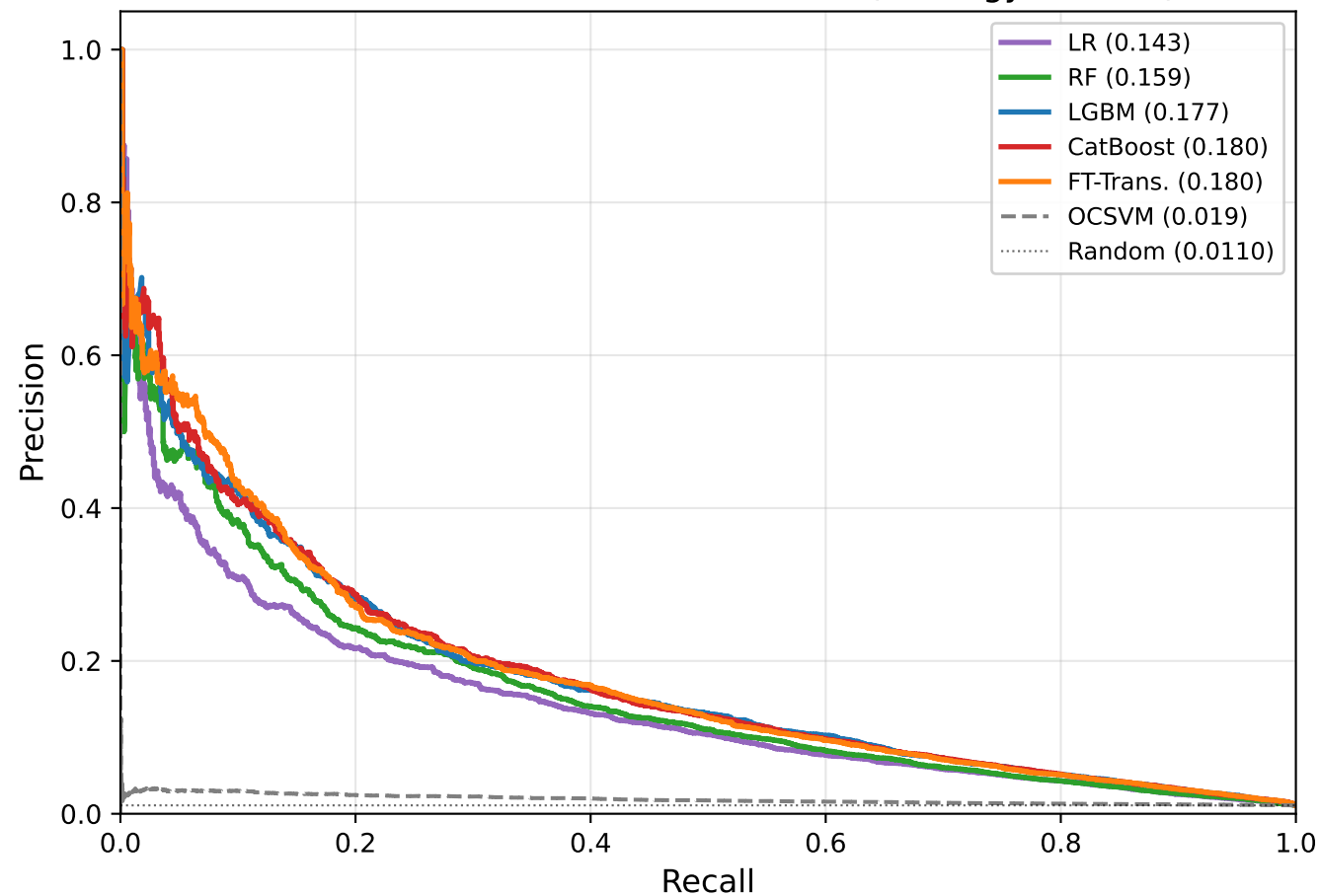
Precision-Recall Curves — BAF Base (strategy = None)
