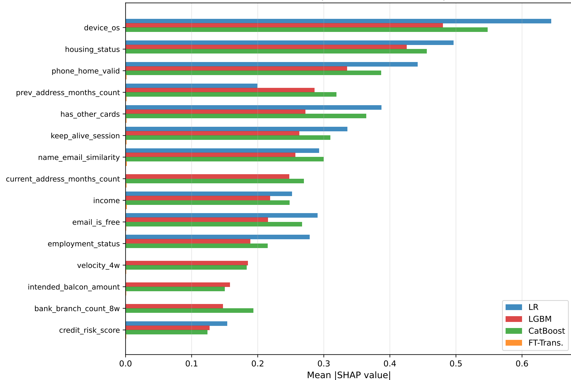
Global Feature Importance (BAF Base, top-15)
