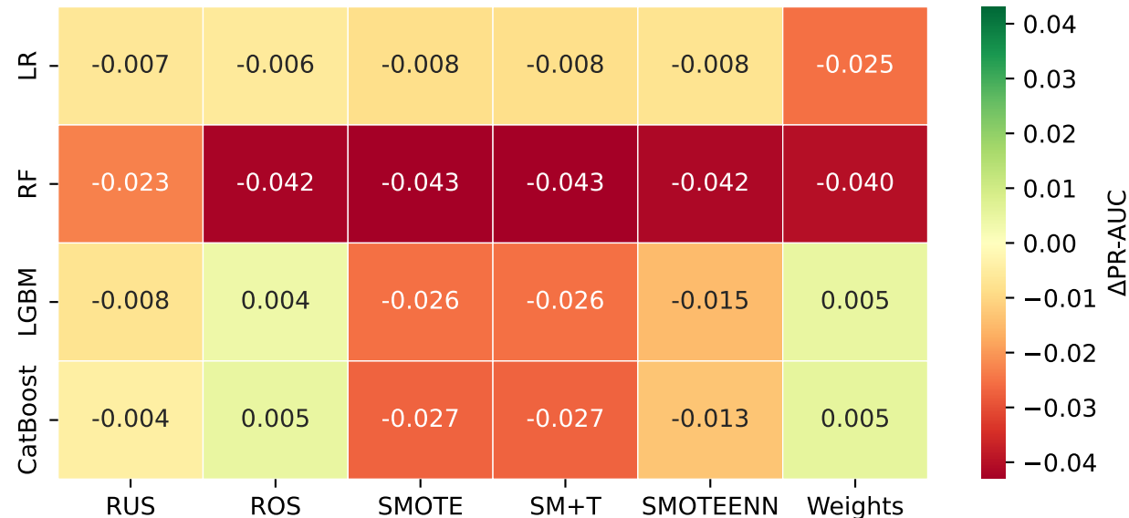
\Delta PR-AUC (strategy – None) — BAF Base
