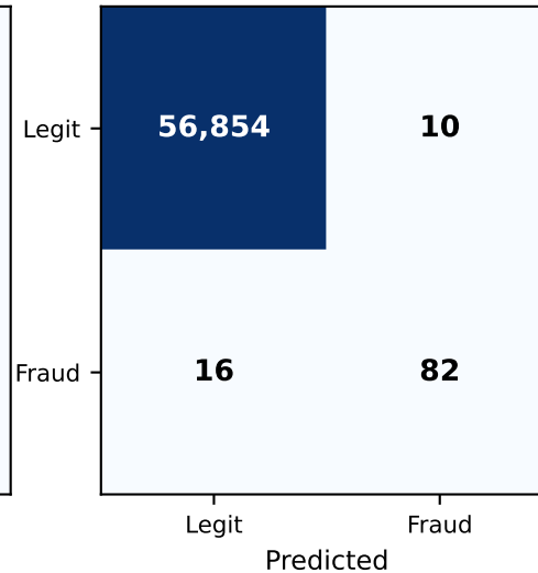
Confusion Matrices — ULB 2013 (strategy = None)
