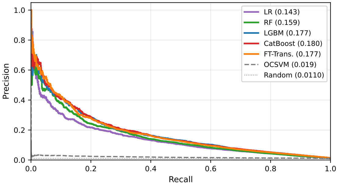
Precision-Recall Curves — BAF Base (strategy = None)
