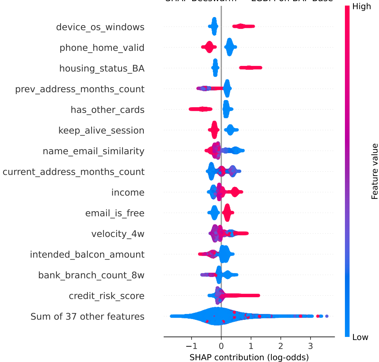
SHAP Beeswarm — LGBM on BAF Base
