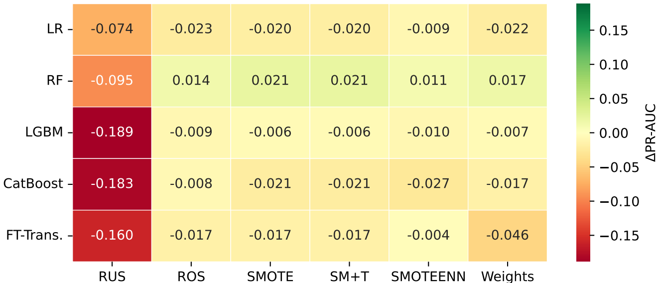
\Delta PR-AUC (strategy – None) — ULB 2013
