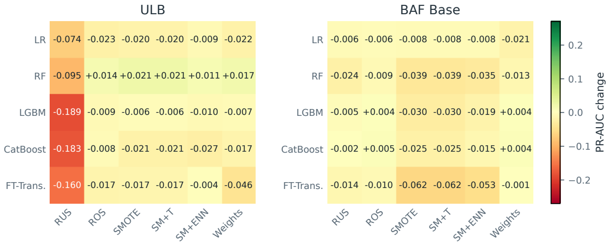
Figure 3: PR-AUC change relative to None on ULB (left) and BAF Base (right). Both panels use the same colour scale. Green indicates improvement and red indicates degradation; SM+ENN denotes SMOTEENN. These are descriptive point-estimate differences for the recorded runs, not significance tests. Plotting code was prepared with OpenAI Codex assistance and uses the saved experimental records.
