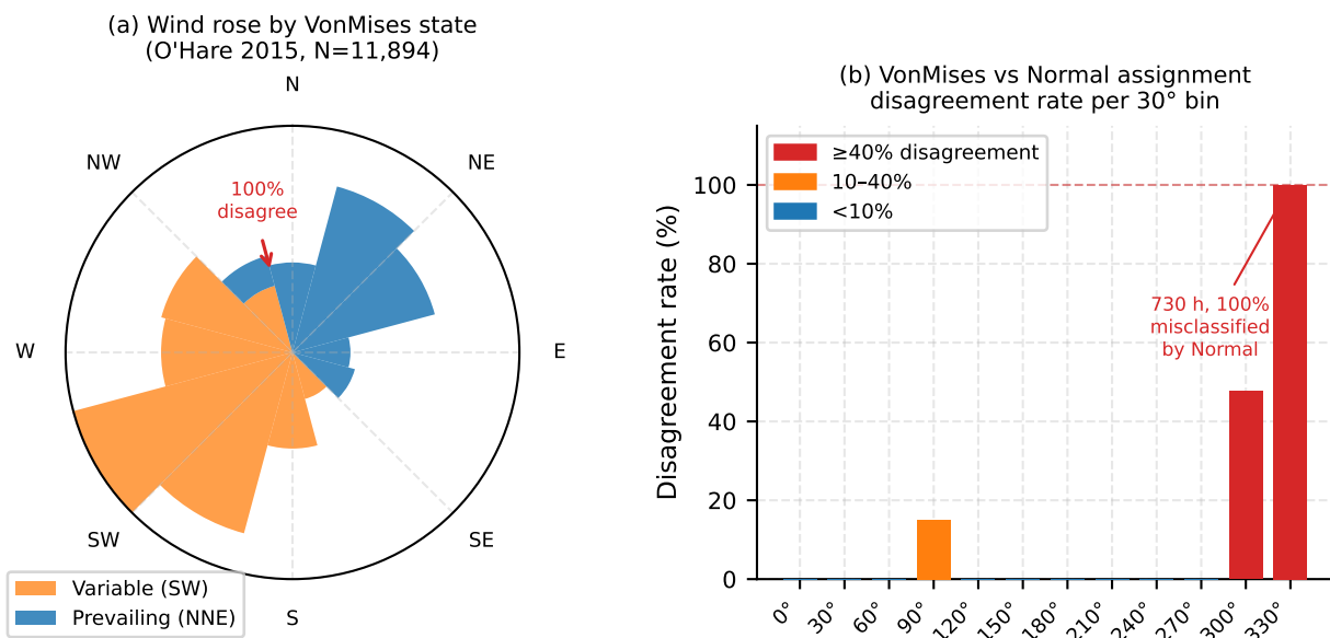
Figure 3 VonMisesDistribution vs Normal approximation — boundary failure at 0^\circ/360^\circ
