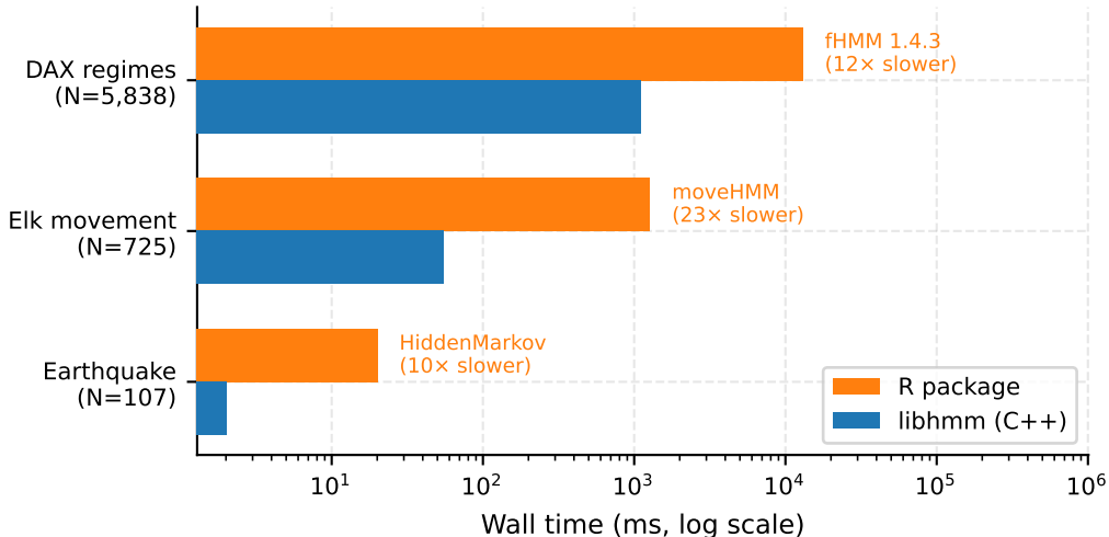
Figure 1 Wall-time comparison: libhmm vs R packages
