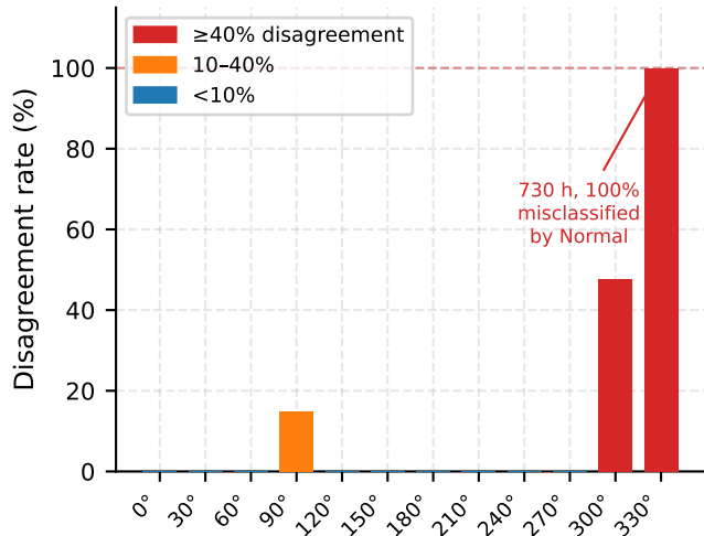
(b) VonMises vs Normal assignment disagreement rate per 30° bin
