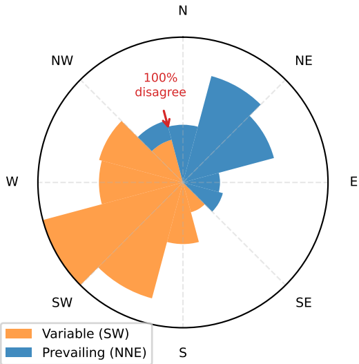
(a) Wind rose by VonMises state (O'Hare 2015, N=11,894)
