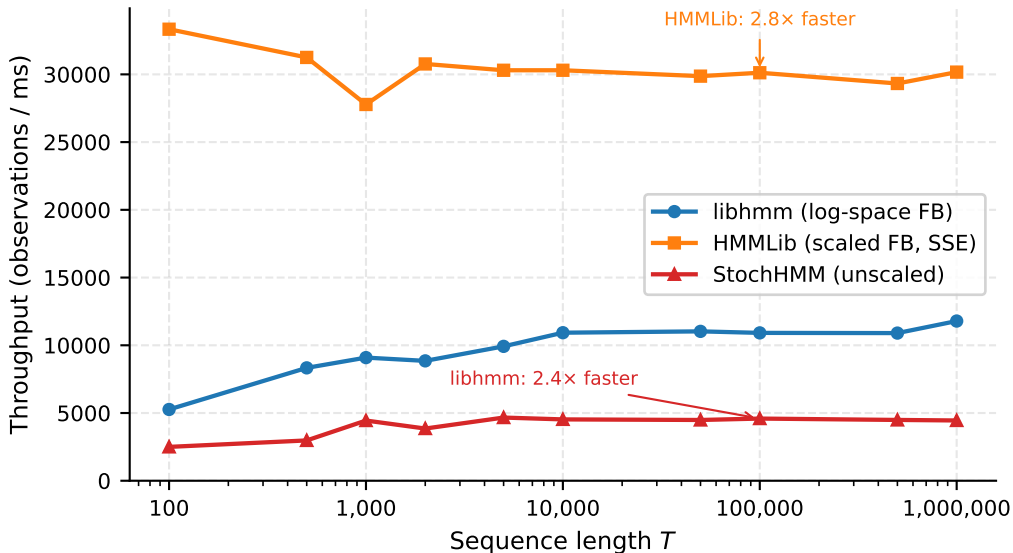
Figure 4 Forward-backward throughput: libhmm vs HMMLib vs StochHMM (Dishonest Casino, 2-state discrete HMM, Windows Ryzen 9 / AVX-512 / MSVC)
