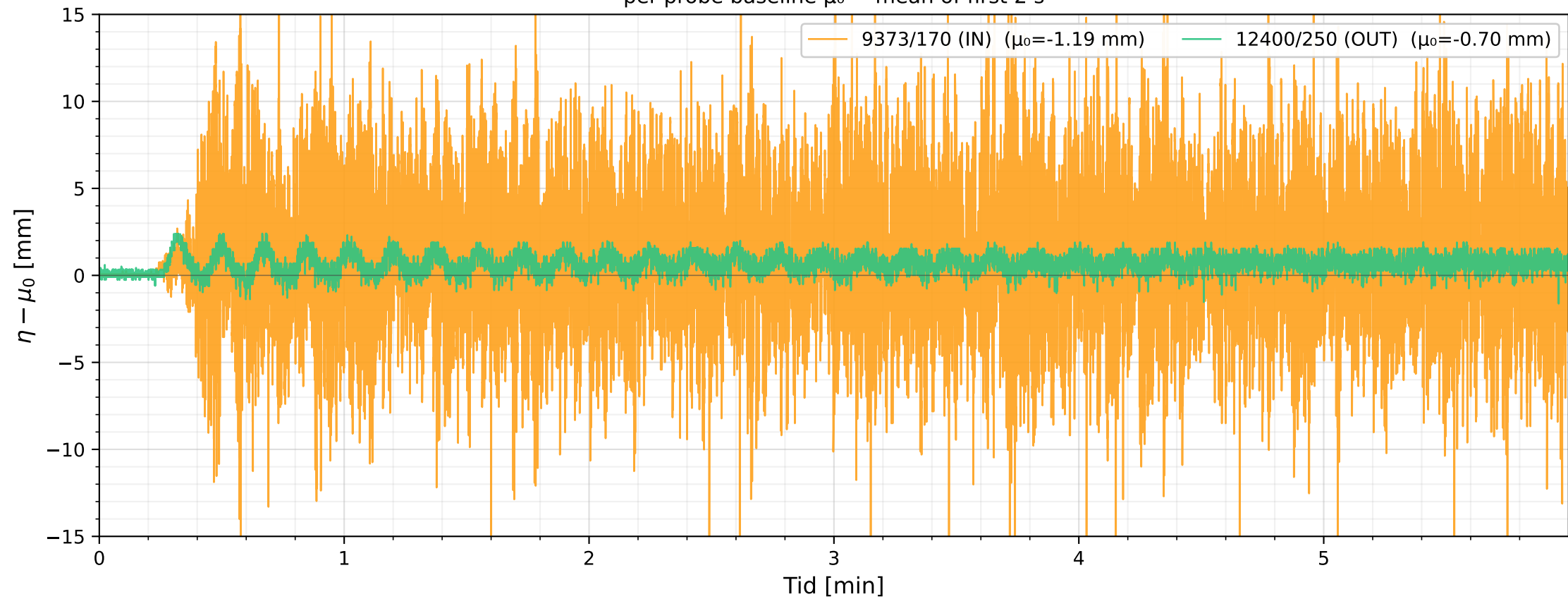
Wind ramp-up — full record (360.0 s = 6.00 min) — 20260314 — fullpanel-fromZeroWinToMaxWin-run1.csv per-probe baseline \mu_0 = mean of first 2 s
