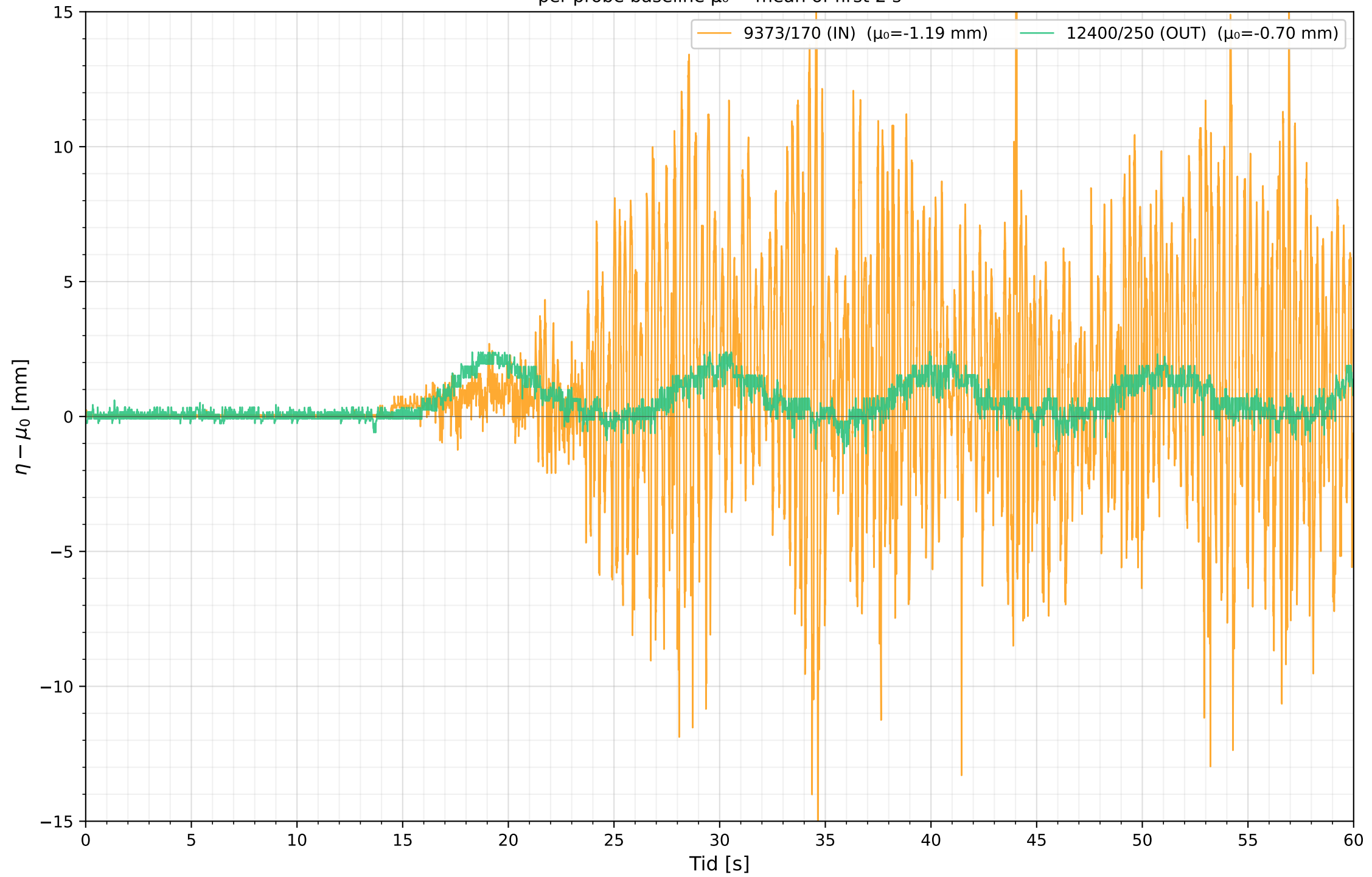
Wind ramp-up — first 60 s — 20260314 — fullpanel-fromZeroWinToMaxWin-run1.csv per-probe baseline \mu_0 = mean of first 2 s
