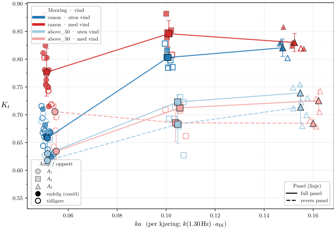
Full vs reverse ved 1.3 Hz — K_t vs ka
