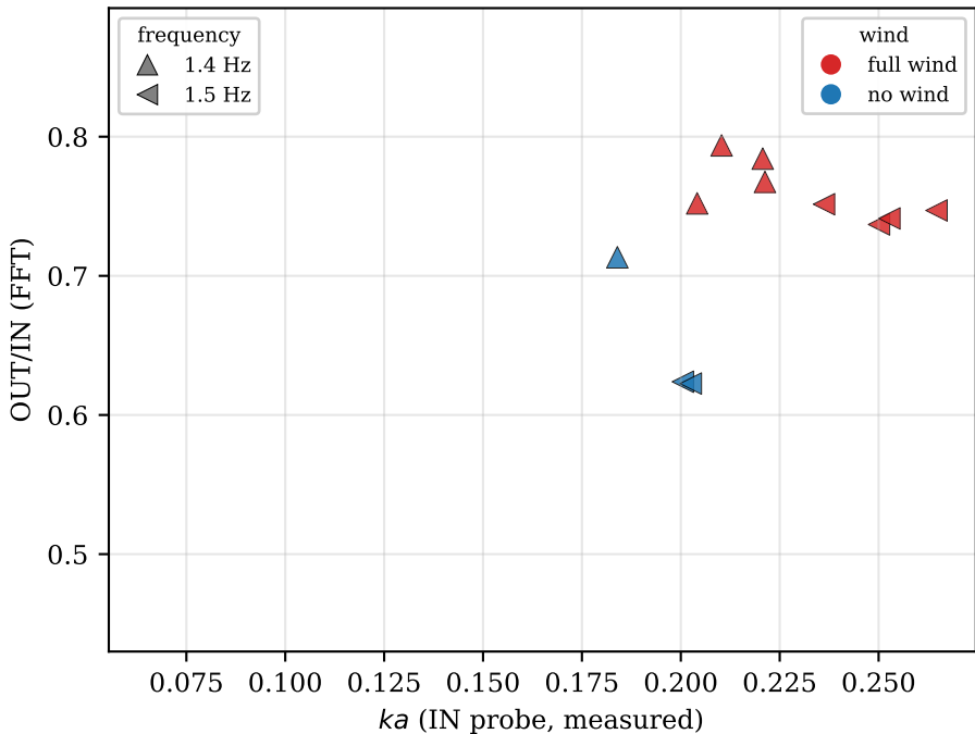
Wave transmission vs. wave steepness — full panel, 0.30 V
