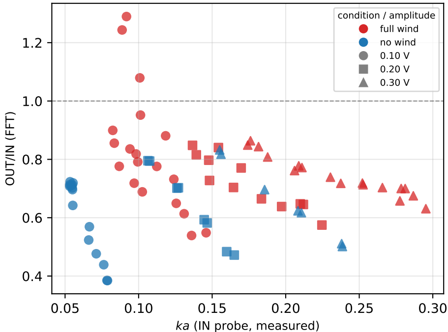
Wave transmission vs. wave steepness — full panel
