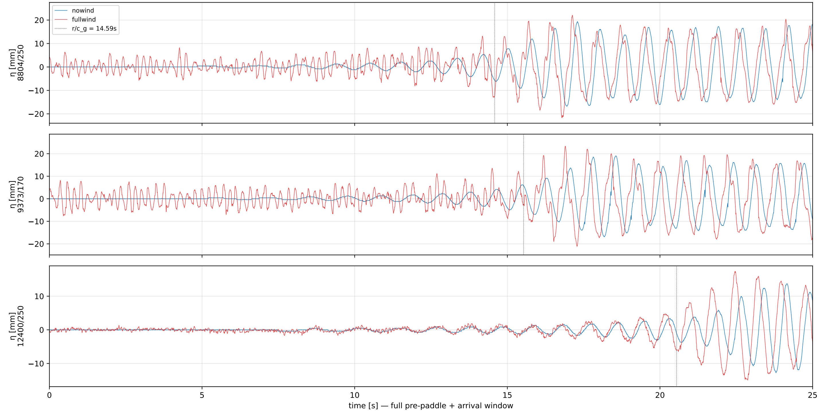
Pre-paddle + first arrival, f=1.3 Hz, A=0.2 V — if paddle starts at same recorded time in fw and nw, any post-arrival \Delta t is propagation/detection
