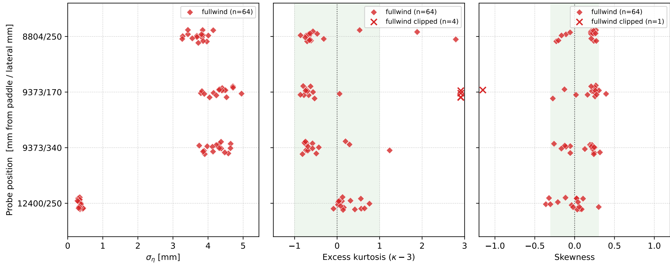
Surface-elevation statistics under wind-only, no-wave runs 16 fullwind runs • no lowestwind+nowave runs in this dataset • trim 5s, fs=250 Hz
