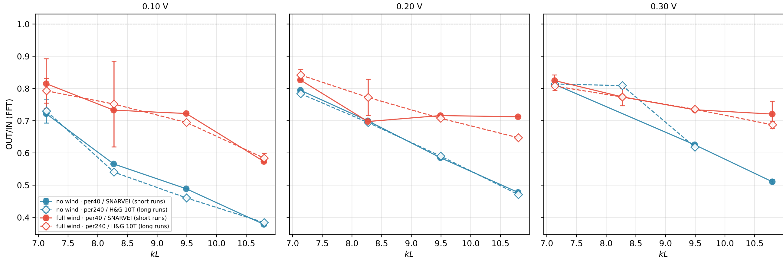
CH04 — OUT/IN (FFT) from short pipeline-SNARVEI windows vs long H&G 10T windows (threshold: N_{\text{input\_periods}} \geq 50 )
