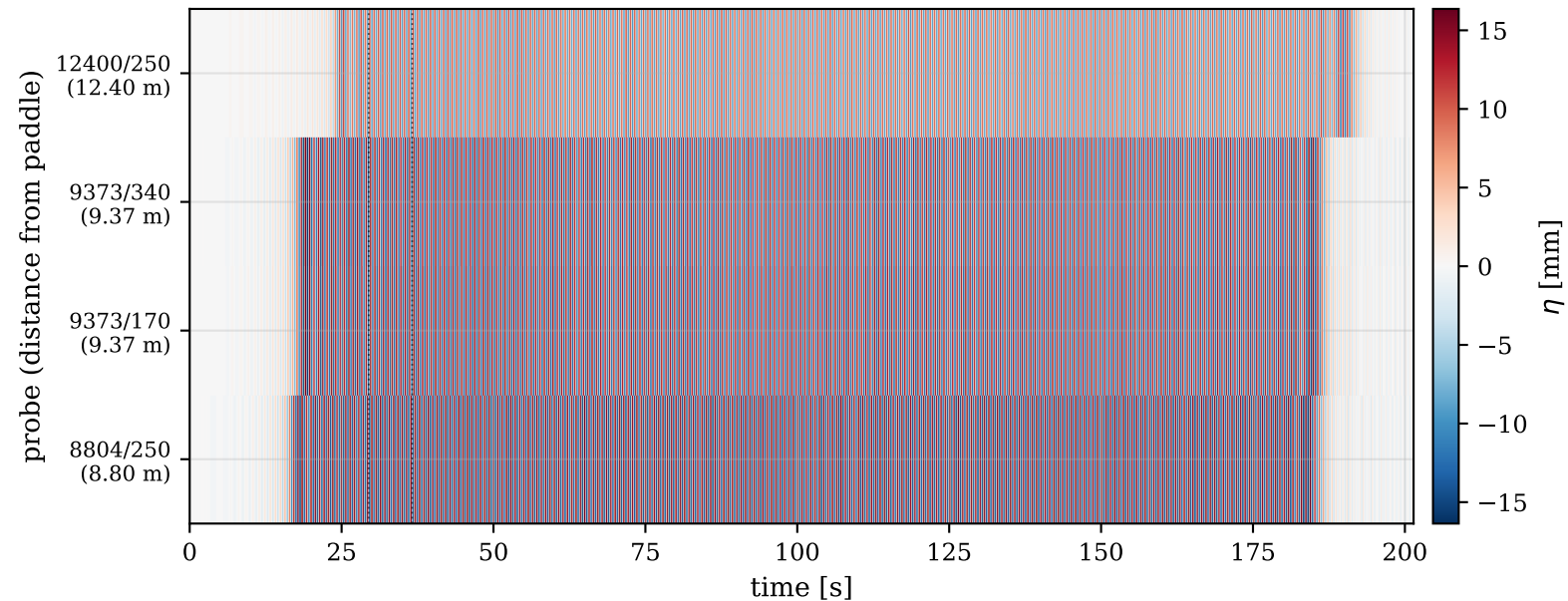
USC Spatiotemporal surface elevation ( f = 1.40 Hz, per240, nowind, fullpanel)
