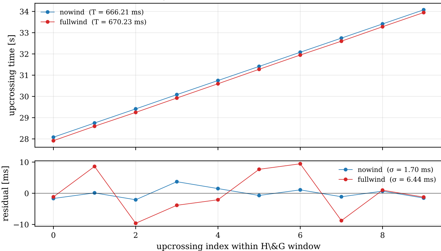
Zero-upcrossing ladder — IN probe (9373/170), f = 1.50 Hz, 0.2 V
