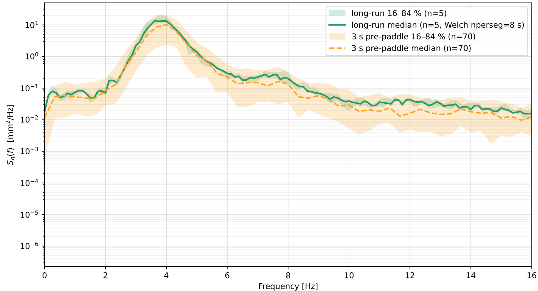
Wind PSD — 5 long nowave runs vs ensemble of 3 s pre-paddle snippets probe 9373/170 (IN, wall) | canon datasets 20260326+27 -lowrange | fullwind
