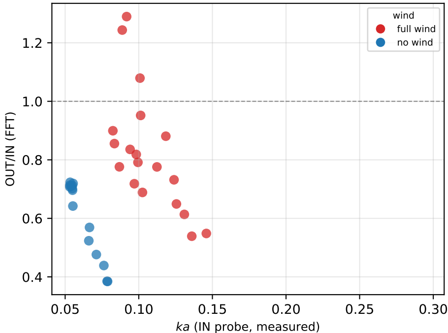
Wave transmission vs. wave steepness — full panel, 0.10 V
