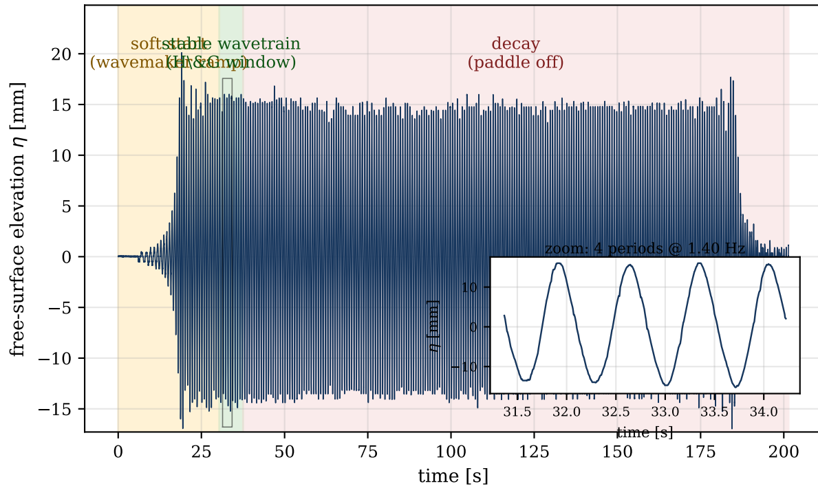
Anatomy of a wave-tank run — probe 9373/170 ( f = 1.40 Hz, per240, nowind, fullpanel)
