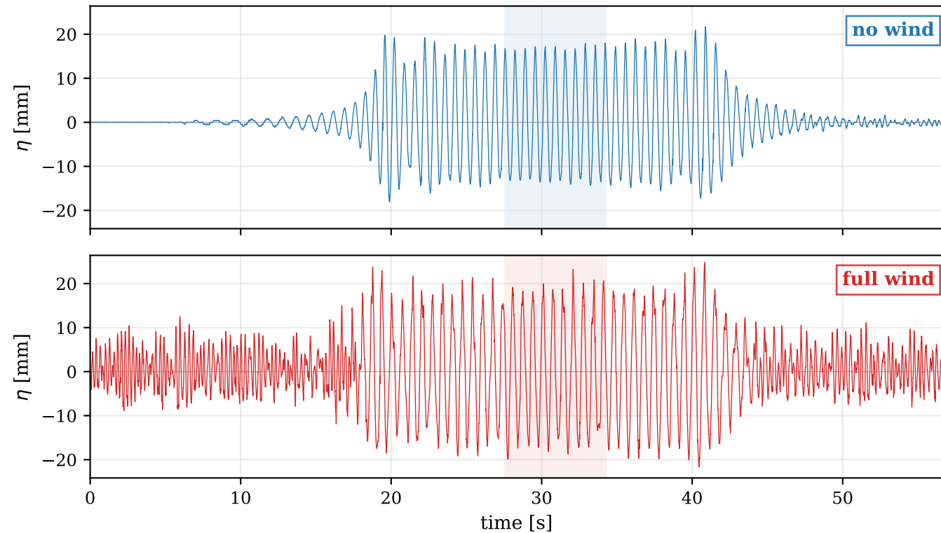
Wind riding on a 1.50\,Hz paddle wave — IN probe 9373/170, per40, 0.2\,V
